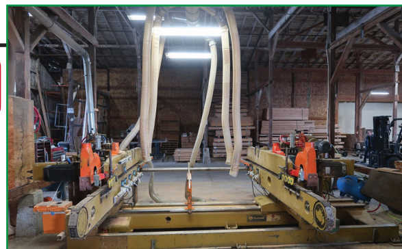
ROCKWELL D80 DOUBLE END TENONER
