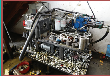
HYDRAULIC PUMP TEST BENCH
