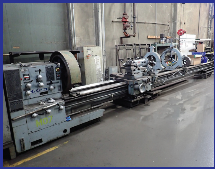
POREBA TPK90A1/8M 36"x30' ENGINE LATHE
