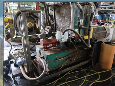
TYRONE BERRY SMA 260 1,500 PSI HYDRAULIC CARRIAGE DRIVE
